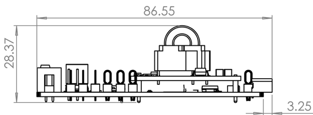
SIDE VIEW (PX OPTION)
