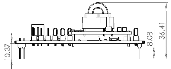
SIDE VIEW (PM OPTION)
